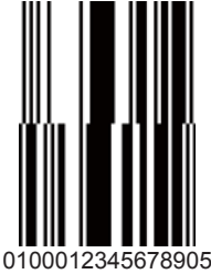
RSS-14/GS1 Databar Limited
